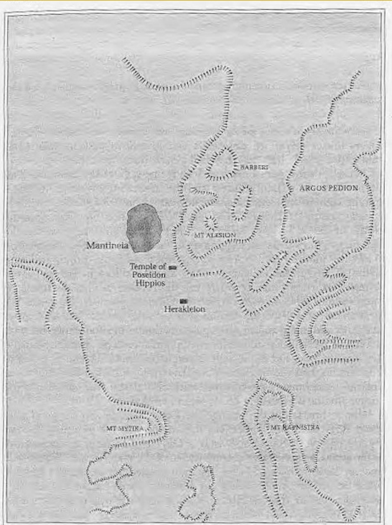
Map 2. Battle of Mantinea Note: the 'Pelagos' wood, south of the temple of Poseidon (Plut. 8. 11. 1) features in some modern reconstructions. But Th. does not mention it, and there is no good reason to suppose that it was relevant to the battle. It is therefore here omitted.
